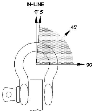
Figure 17 Side Loading
