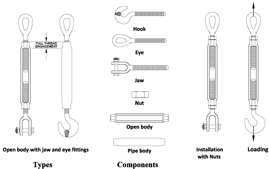
Figure 19 Turnbuckle Types
