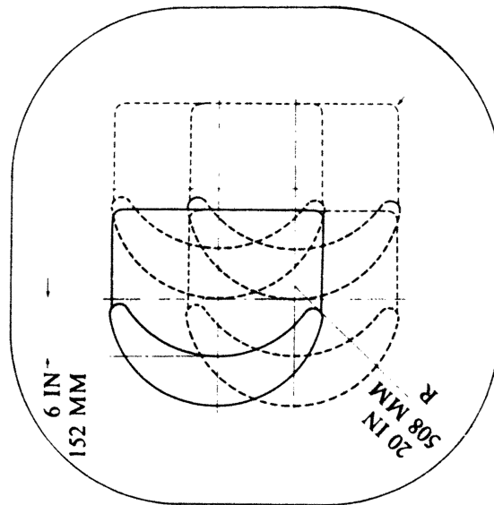
FIGURE V-26 Zone of protection for drop test.
