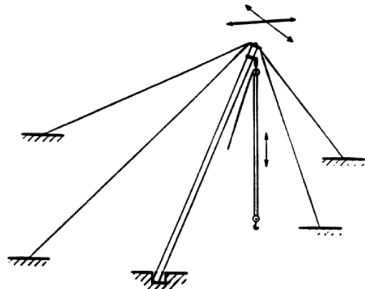
Gin-Pole Derrick
