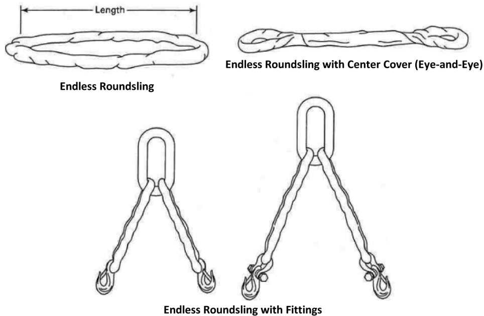
Figure 26 Synthetic Roundslings
