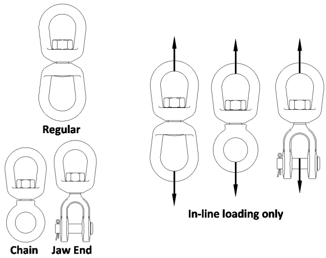
Figure 38 Swivels
