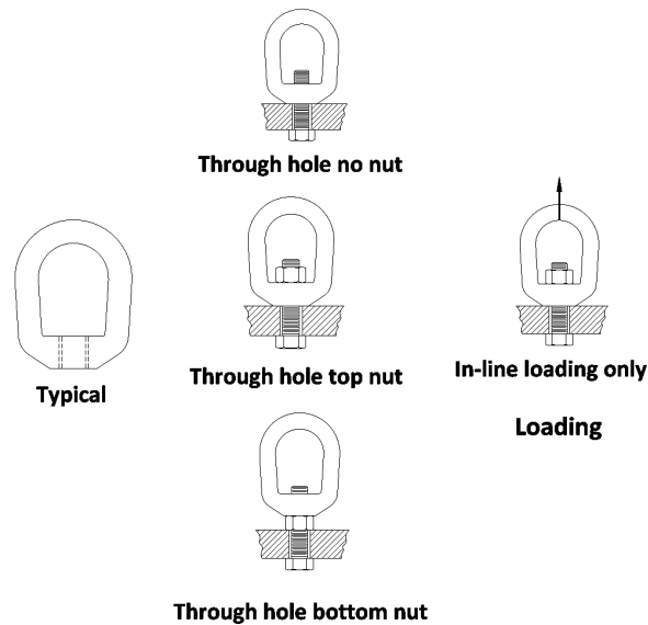
Figure 21 Eye Nuts
