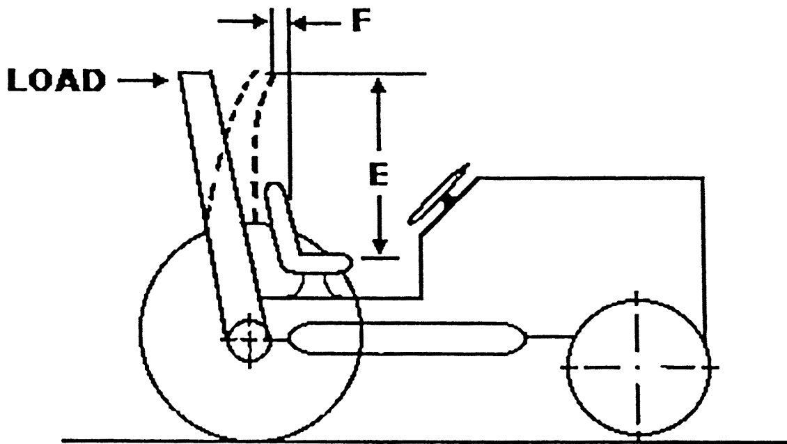
FIGURE V-18 Rear load application.
