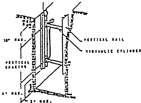
Figure N-23, Aluminum Hydraulic Shoring
