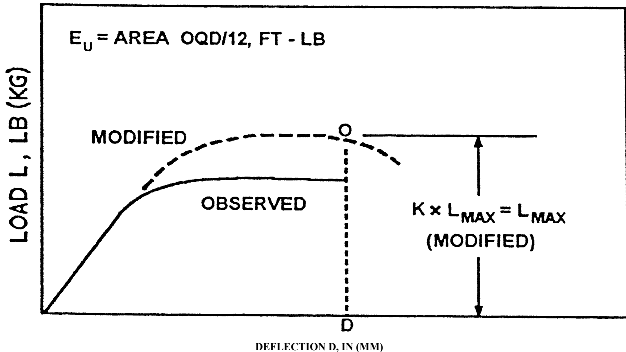
FIGURE V-21 Typical modified L_m - D_m diagram.
