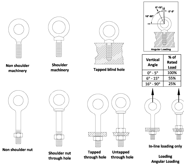
Figure 20 Eyebolts
