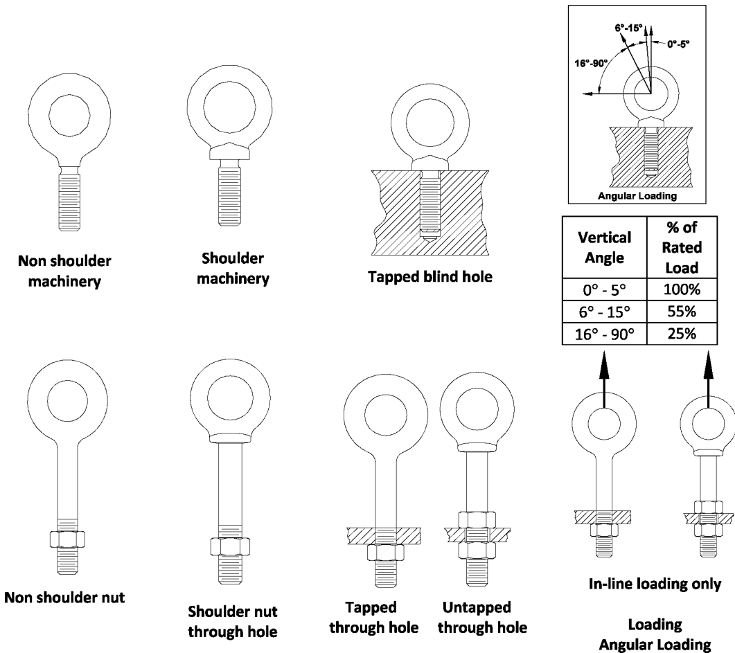
Figure 31 Eyebolts
