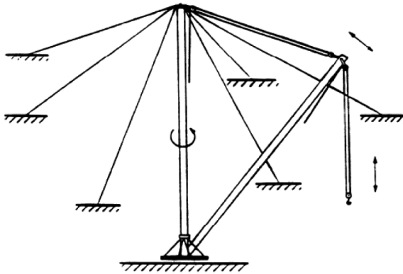
Guyed Derrick
